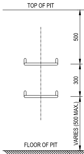
ELEVATION SCALE 1:20
