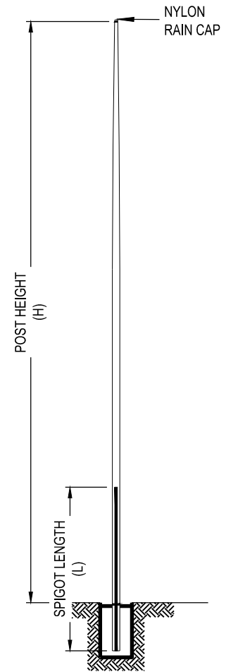
GOAL POST DETAIL NOT TO SCALE
