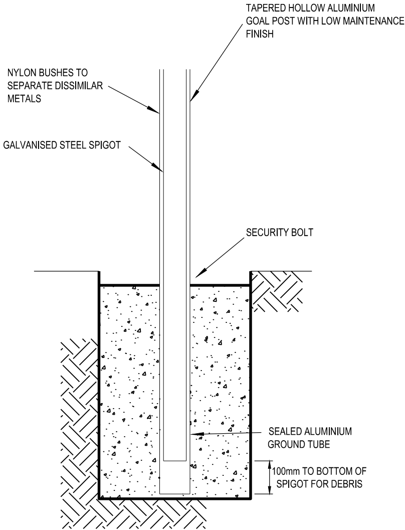
GOAL POST FOOTING NOT TO SCALE
