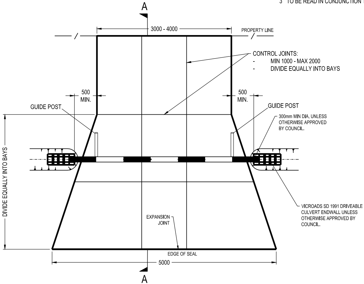
PLAN SCALE 1:50
