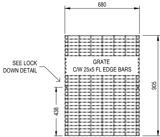
GRATE DETAIL
