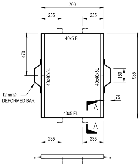
FRAME DETAIL
