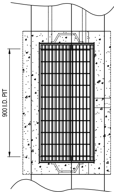
PLAN
