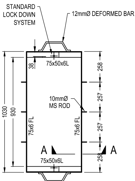
FRAME
