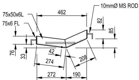
FRAME DETAIL
