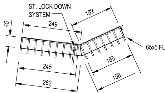
GRATE DETAIL
