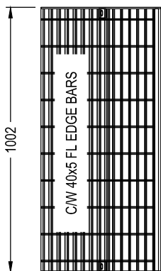
GRATE
