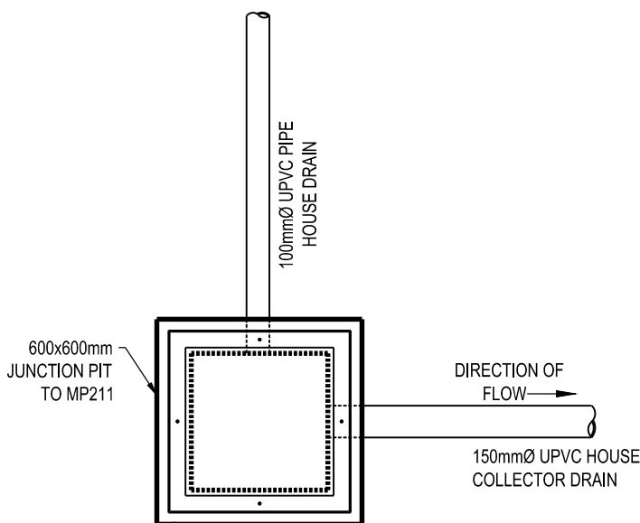
DETAIL OF UPSTREAM END OF COLLECTOR DRAIN NOT TO SCALE
