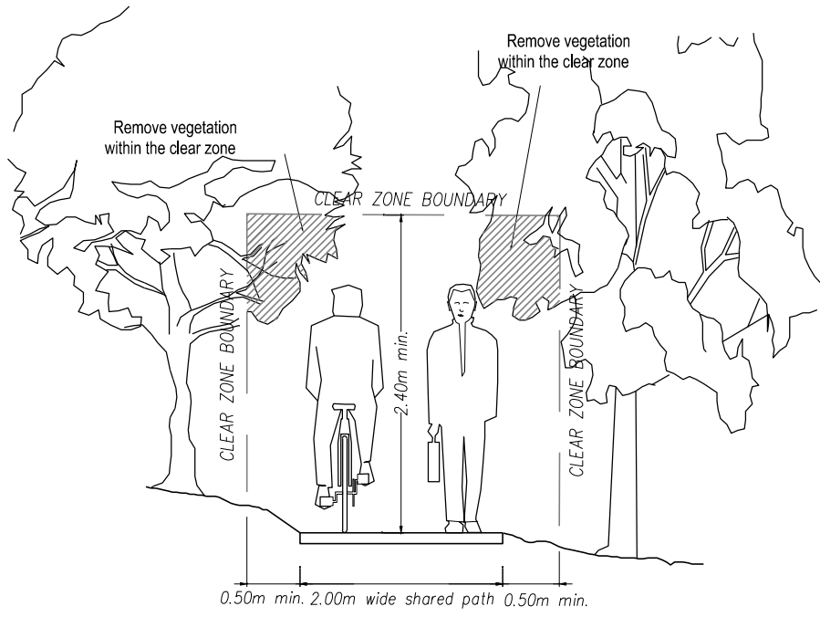
PEDESTRIAN / BICYCLE CLEAR ZONE NOT TO SCALE
