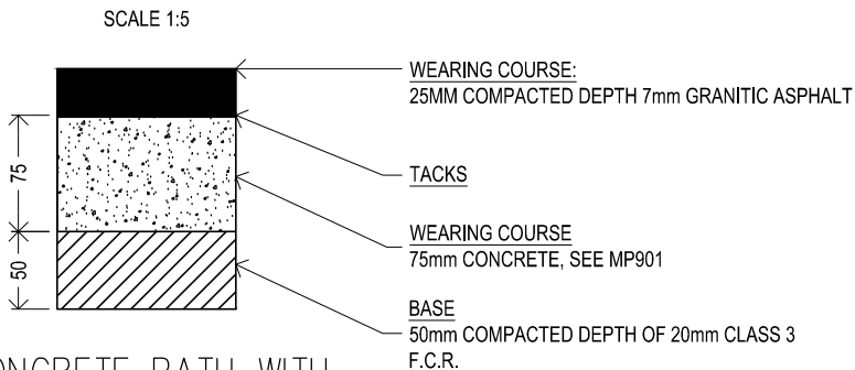
CONCRETE PATH WITH ASPHALT WEARING COURSE
