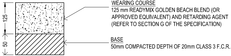
EXPOSED AGGREGATE CONCRETE
