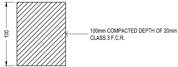
CRUSHED ROCK
