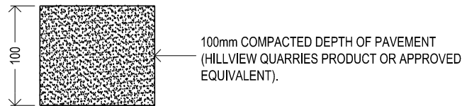
GRANITIC SAND
