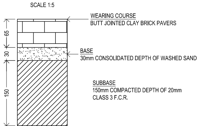
BRICK PAVED
