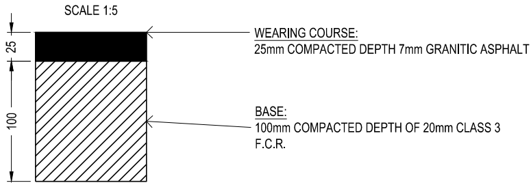
GRANITIC ASPHALT
