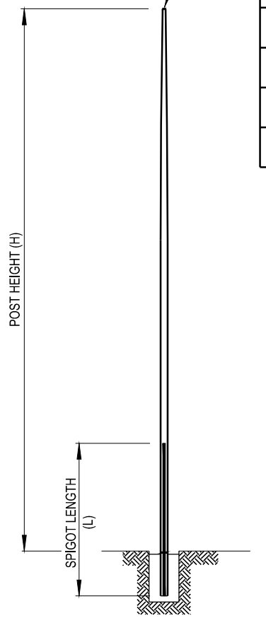
GOAL POST DETAIL NOT TO SCALE
