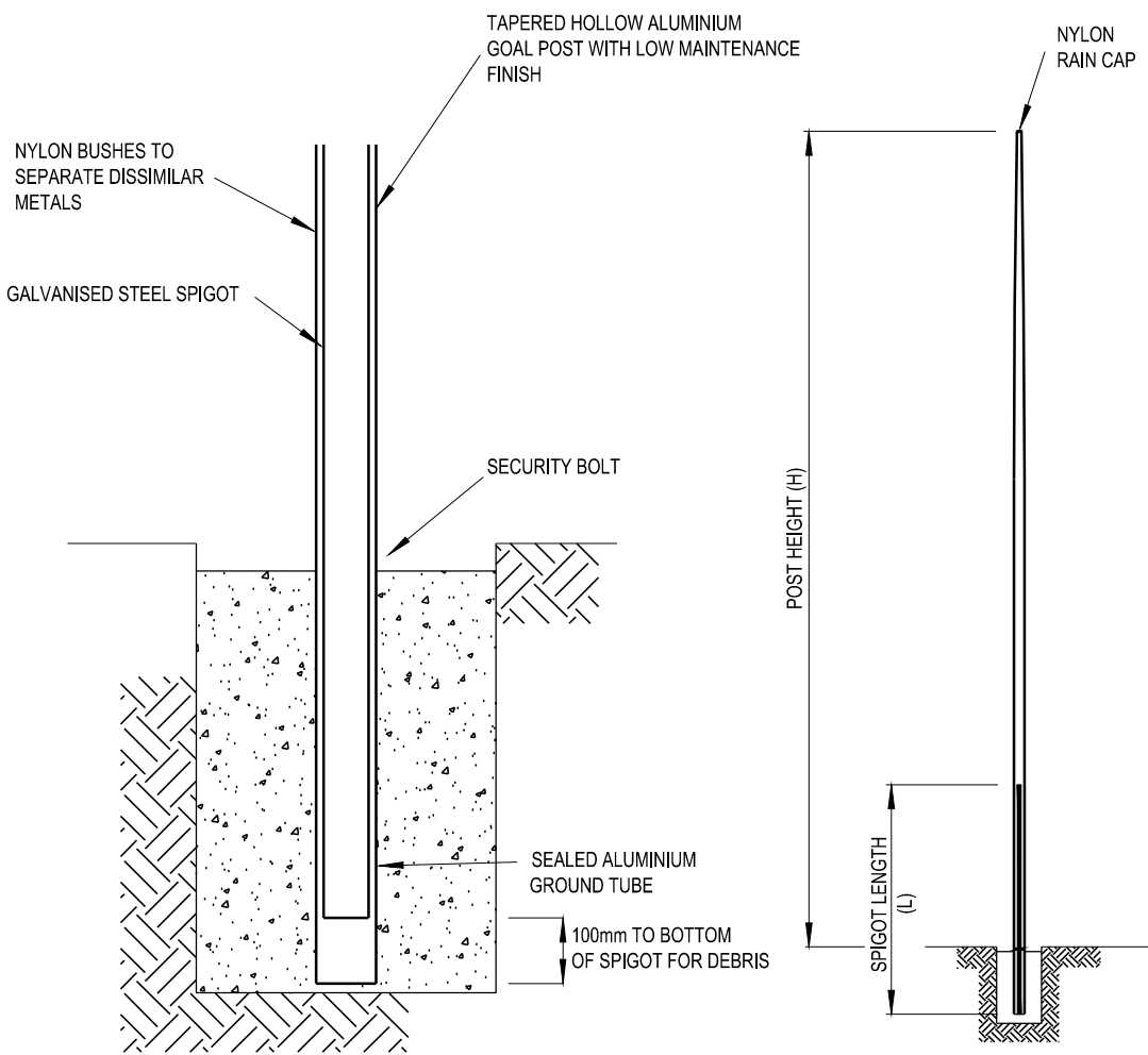
GOAL POST DETAIL NOT TO SCALE
