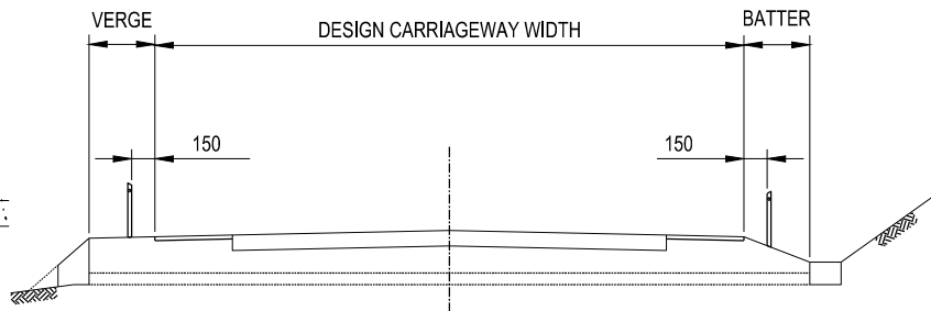
LATERAL LOCATION OF GUIDE POSTS SCALE 1:50
