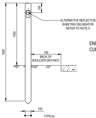
(III) FLEXIBLE POST NOT TO SCALE
