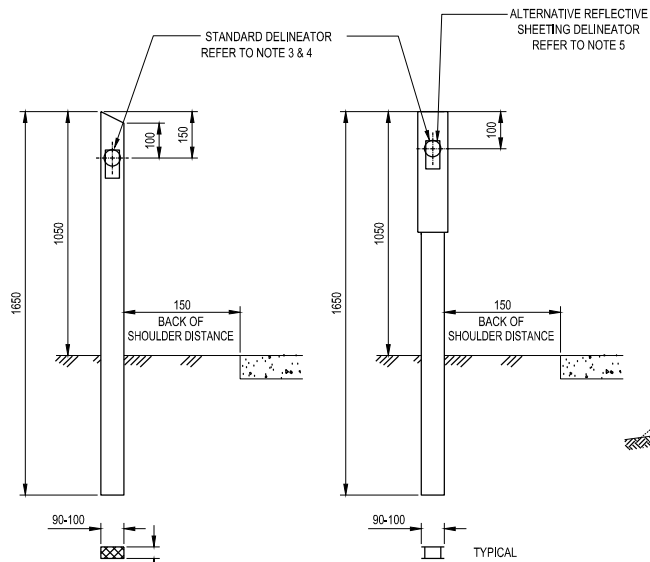
(I) TIMBER POST NOT TO SCALE
