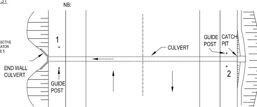
LOCATION OF CULVERT GUIDE POSTS SCALE 1:50
