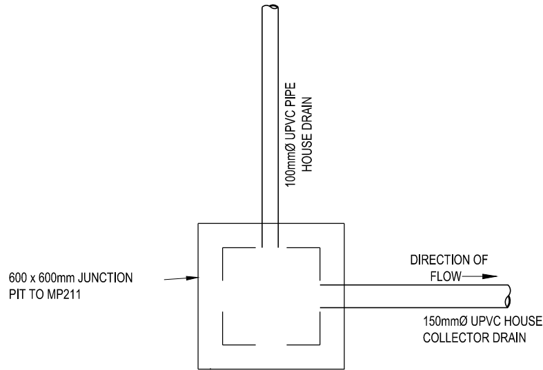
DETAIL OF UPSTREAM END OF COLLECTOR DRAIN NOT TO SCALE
