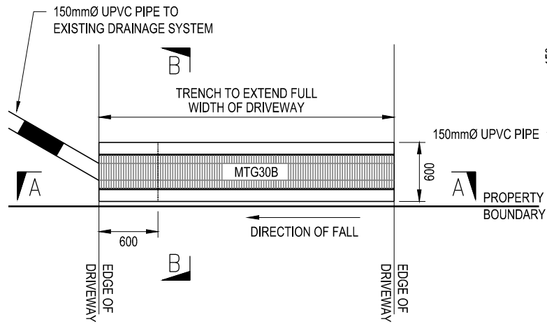
TRENCH & TRENCH GRATE DETAIL
