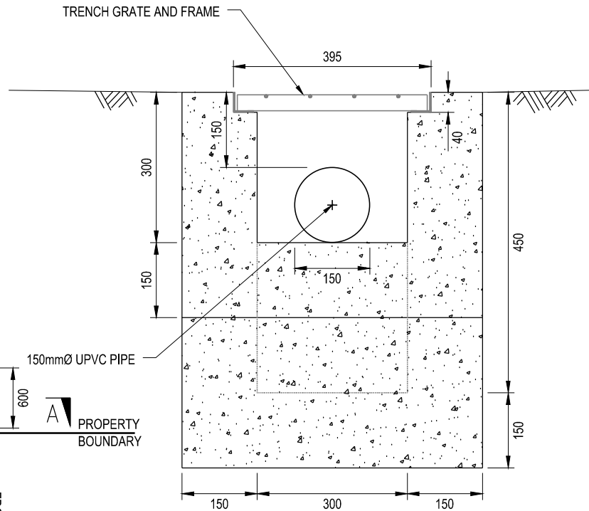
SECTION B-B
