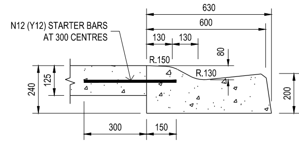
SECTION A-A ROLLOVER KERB & CHANNEL NOT TO SCALE
