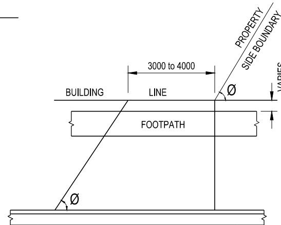
SKEW CROSSING NOT TO SCALE
