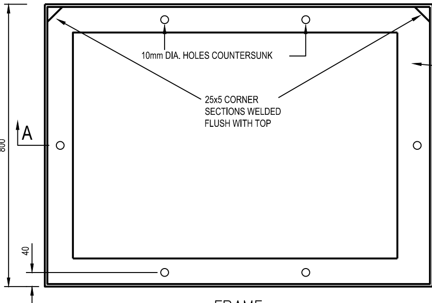
FRAME SCALE 1:10
