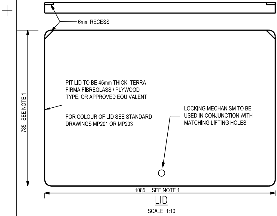
FRAME SCALE 1:10
