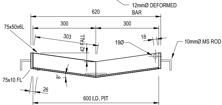
FRAME DETAIL
