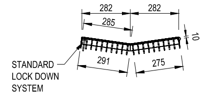
GRATE DETAIL
