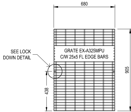
GRATE DETAIL SCALE 1:10
