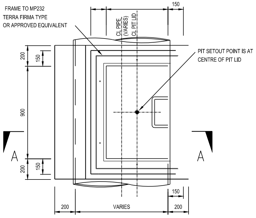
MAIN DRAIN INSPECTION MANHOLE SCALE 1:20
