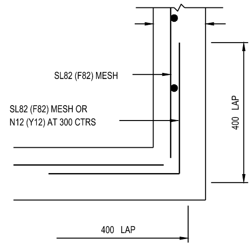
PLAN OF CORNER DETAIL SCALE 1:10
