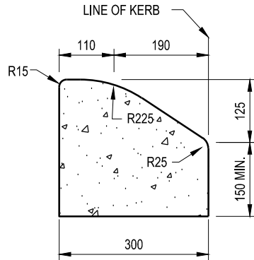
SEMI-MOUNTABLE KERB (IN PAVEMENT) FOR ROUNDABOUTS AND ISLANDS
