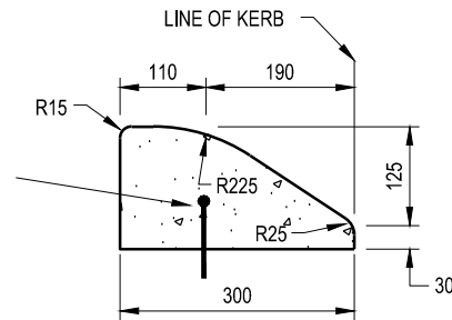
SEMI-MOUNTABLE KERB (SPIKED) FOR ROUNDABOUTS AND ISLANDS
