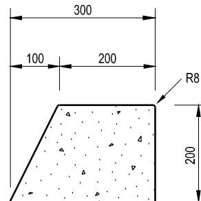
CONCRETE EDGE STRIP FOR BRICK PAVING
