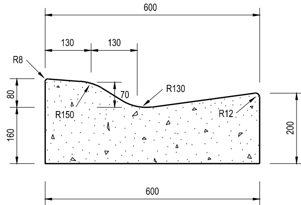
ROLLOVER KERB & CHANNEL FOR BRICK PAVING
