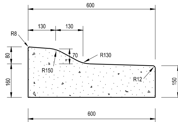
ROLLOVER KERB & TRAY FOR BRICK PAVING
