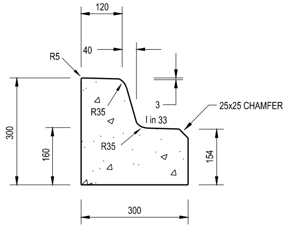
BARRIER KERB FOR ONEWAY CROSSFALL
