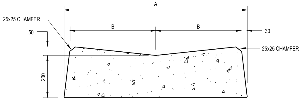
OPEN INVERT CHANNEL
