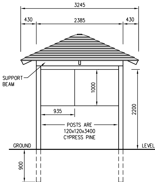
FRONT VIEW SCALE 1:50
