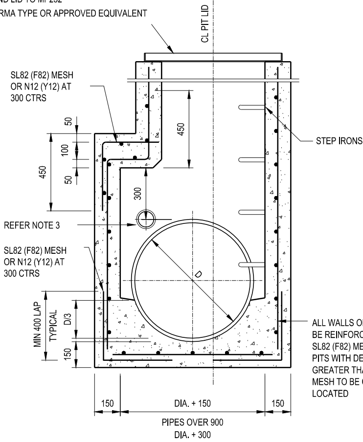
TYPICAL SECTION SCALE 1:20
