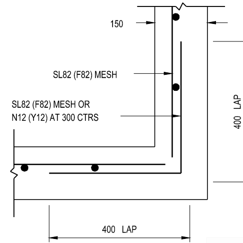
PLAN OF CORNER DETAIL SCALE 1:10
